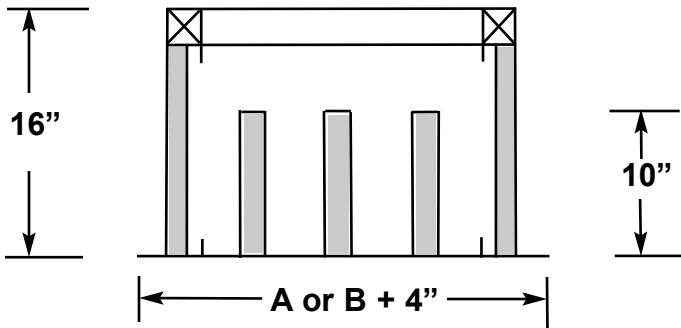
Elevation/Section View
